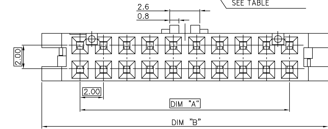
VIEW WITHOUT COVER
